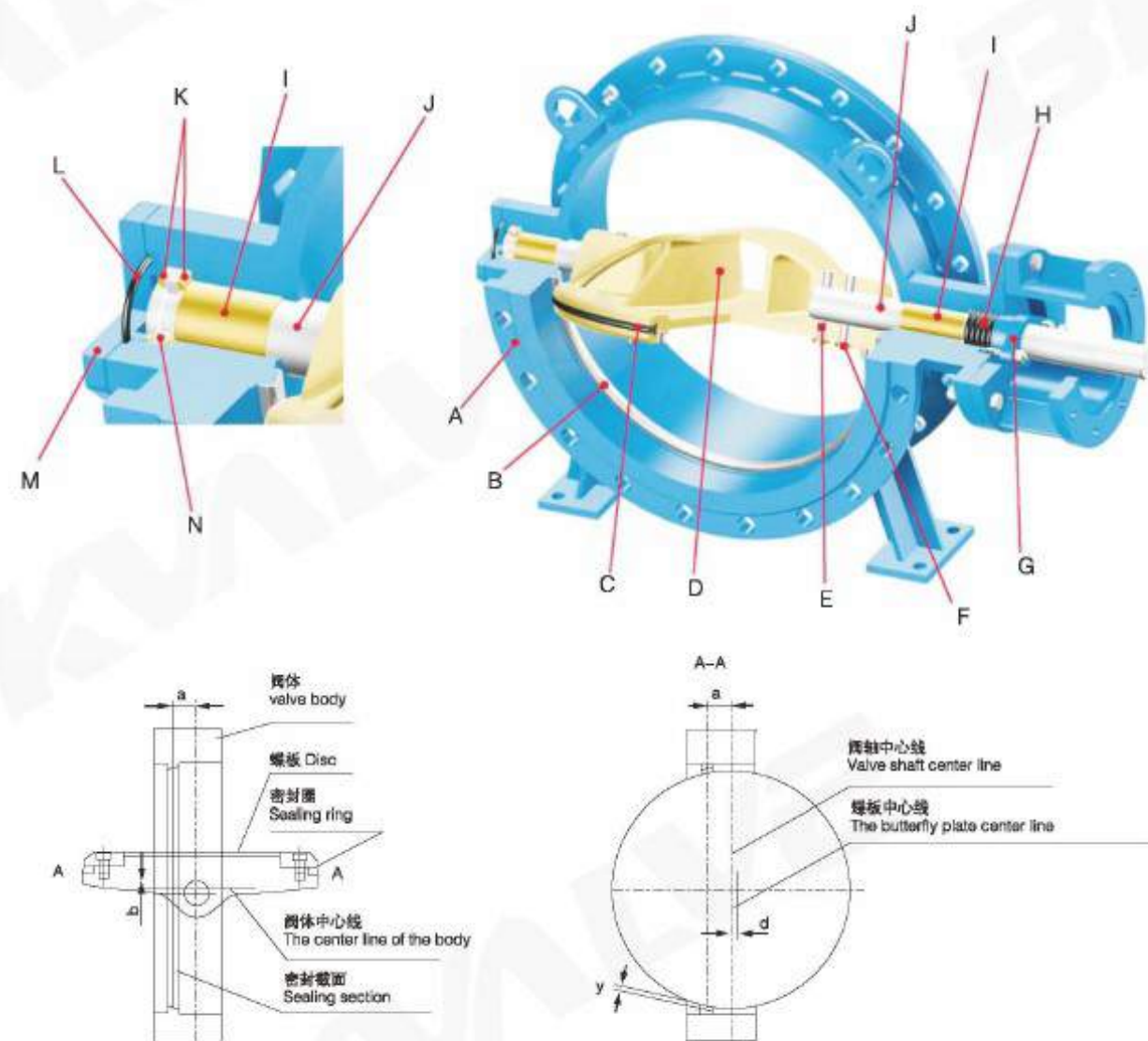
双偏心密封蝶阀密封结构 Double eccentric butterfly valve seal structure
